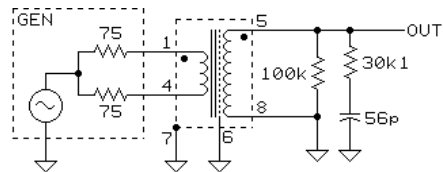
TEST CIRCUIT 2
