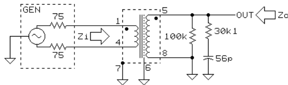
TEST CIRCUIT 1
