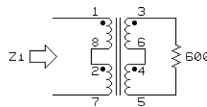
TEST CIRCUIT 3
