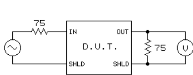
TEST CIRCUIT 1
