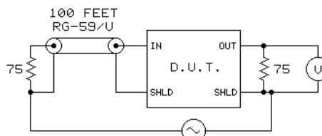
TEST CIRCUIT 2
